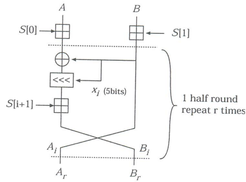
Fig. 1. RC5 encryption algorithm
